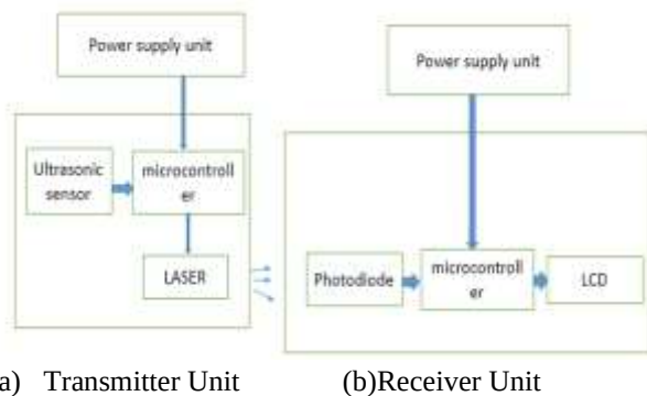
Figure 3: Block Diagram of the Li-Fi Concept for V2V Communication
