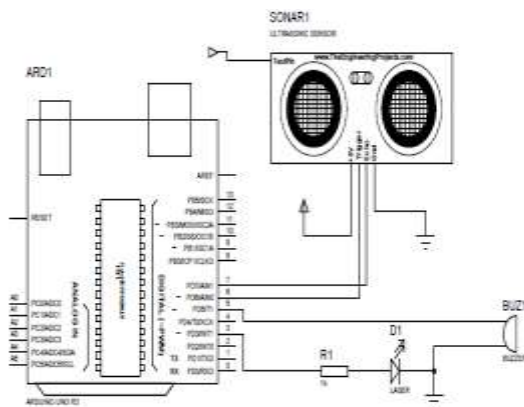
(a) Transmitter Circuit Diagram
