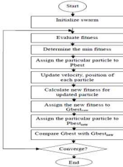
Fig..3 . General Flow Chart of the PSO
