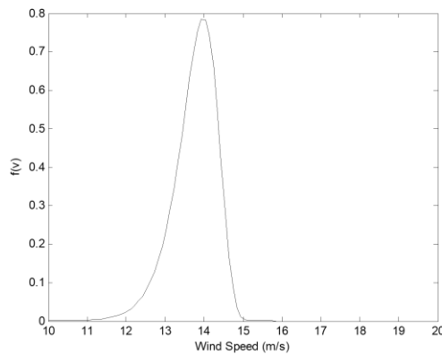
Figure3: Weibull probability density function
