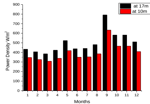
Figure 5: Wind power density at 17m and 10m heights
