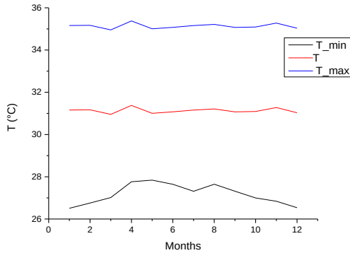
Figure 6: Average Temperature, Minimum Temperature and Maximum Temperature over the three years.
