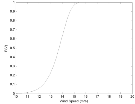
Figure 4: Weibull cumulative probability distribution for wind speed
