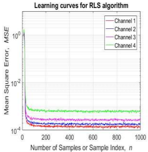
Fig. 2. Learning Curves for RLS under different channel conditions
