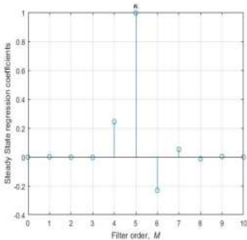
Fig. 5. Steady-state regression coefficients of RLSL for filter order M = 1
