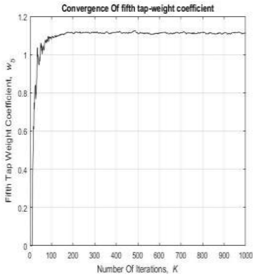
Fig. 4. The convergence of RLS tap weight coefficient for channel 1.
