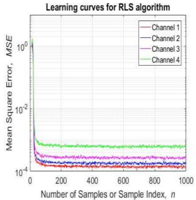
Fig. 2. Learning Curves for RLS under different channel conditions
