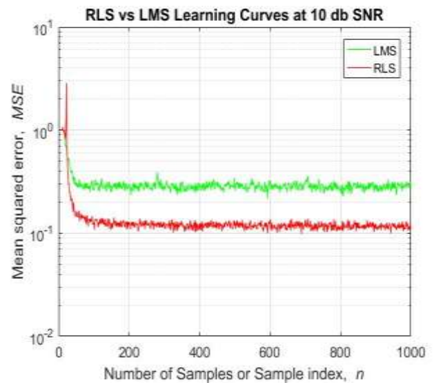
Fig. 3. RLS vs LMS Performance for small SNR regime.
