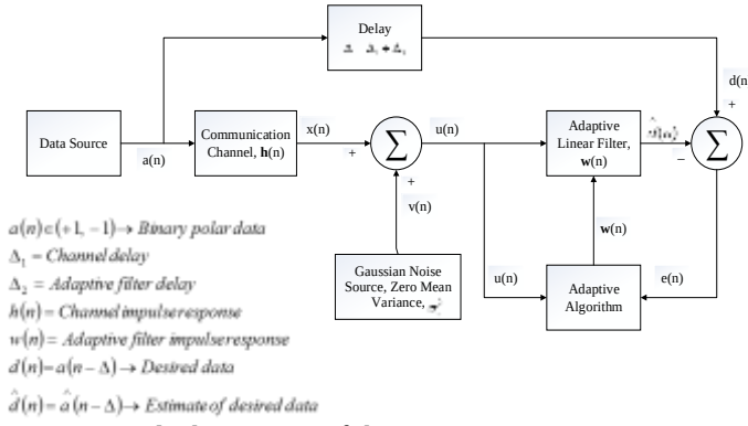
Fig. 1. Block Diagram of the communication system showing the adaptive equalization stage
