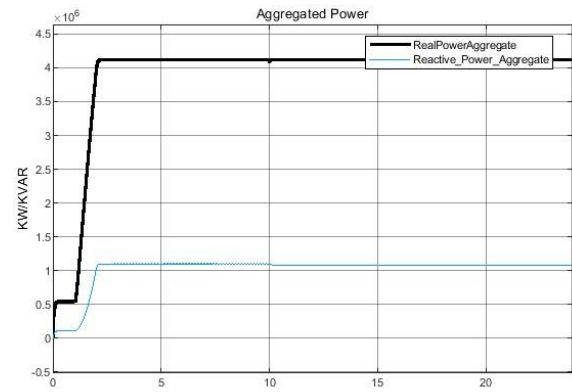
Fig. 15 Aggregate power transmitted to loads
