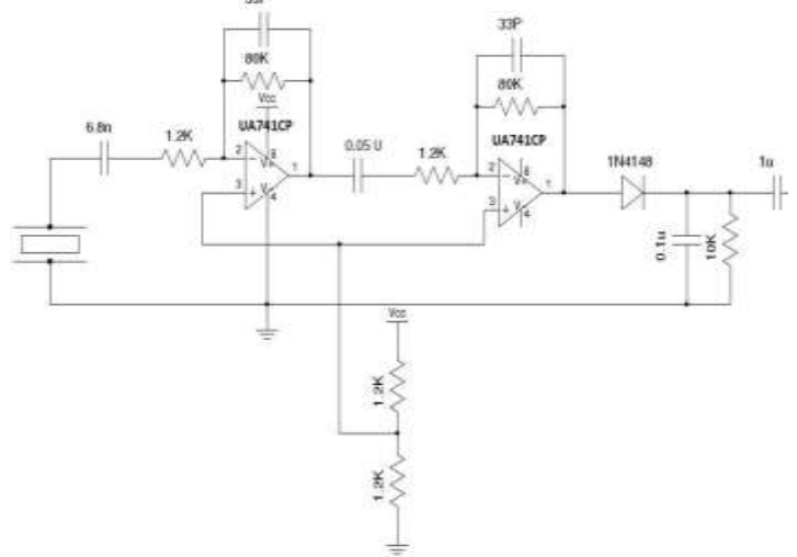
Figure 3: Internal Structure of Receiver Circuit of the HC-SR04 Ultrasonic Sensor
