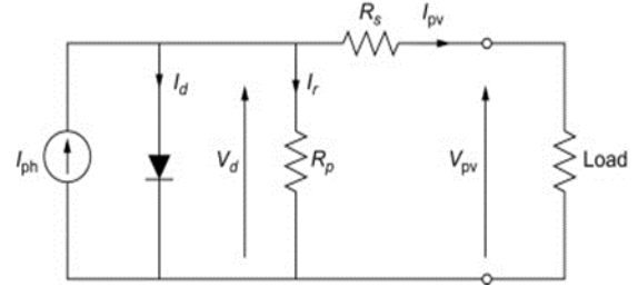
Figure 2: PV Model Electrical equivalent circuit
