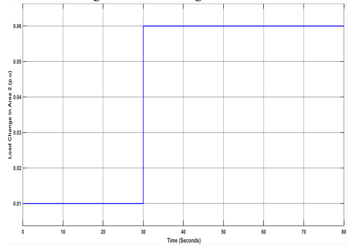
Figure 4: Load Change in Area 2
