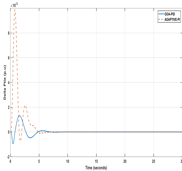
Figure 12: Change in Frequency deviation in Power tie-line
