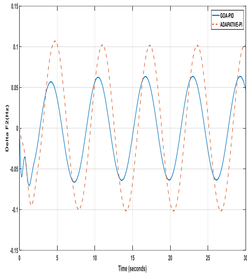
Figure 9: Change in Frequency deviation in Area 2
