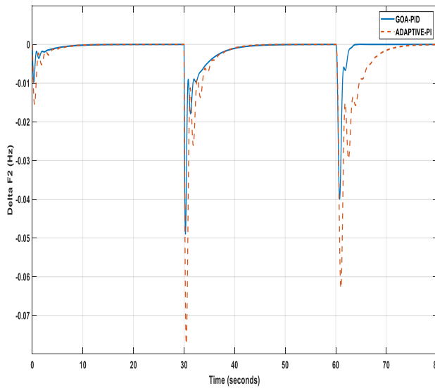
Figure 6: Change in Frequency deviation in Area 2
