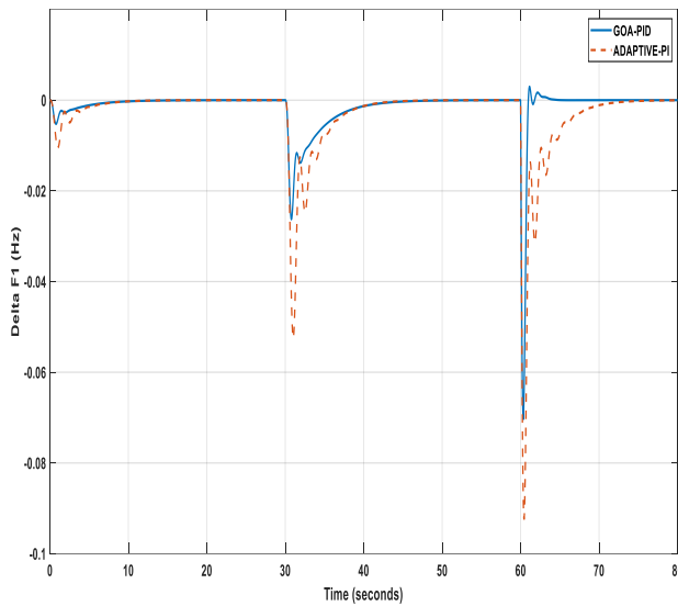
Figure 5: Change in Frequency deviation in Area 1
