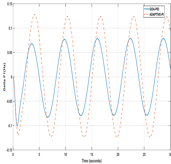
Figure 8: Change in Frequency deviation in Area 1
