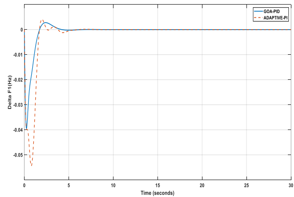
Figure 10: Change in Frequency deviation in Area 1
