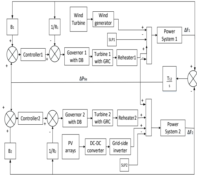
Figure 1: Two-area network integrated with renewable energy sources model
