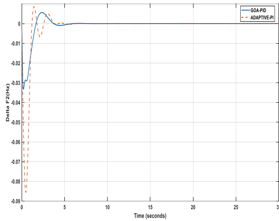
Figure 11: Change in Frequency deviation in Area 2
