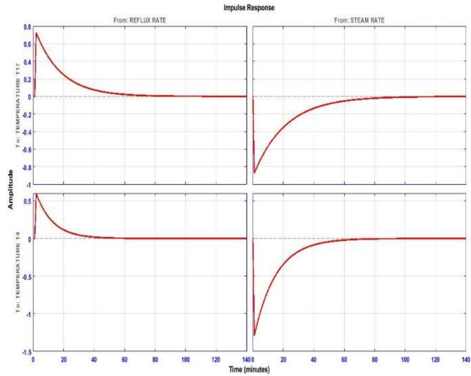
Figure 5: Impulse Response of the System.
