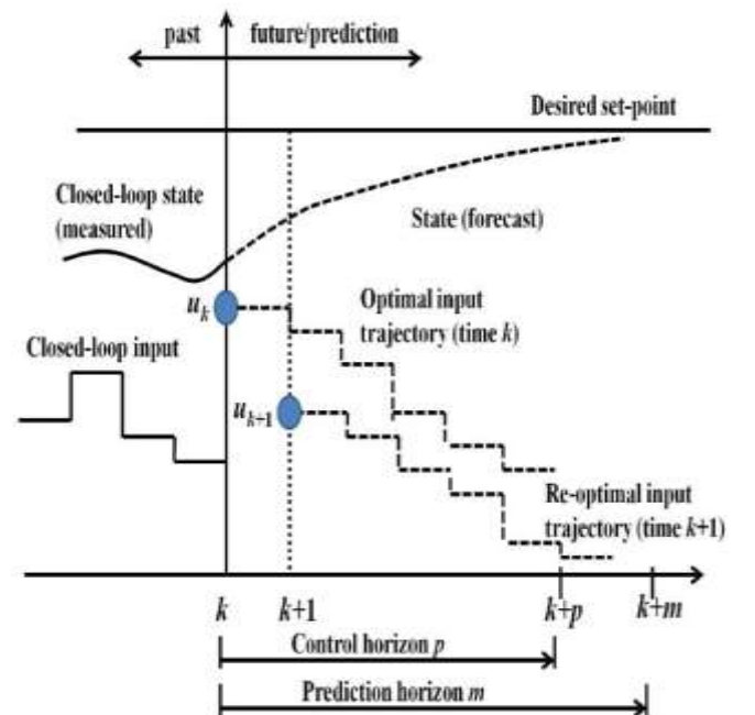
Figure 2: Model Predictive Control Representation.
