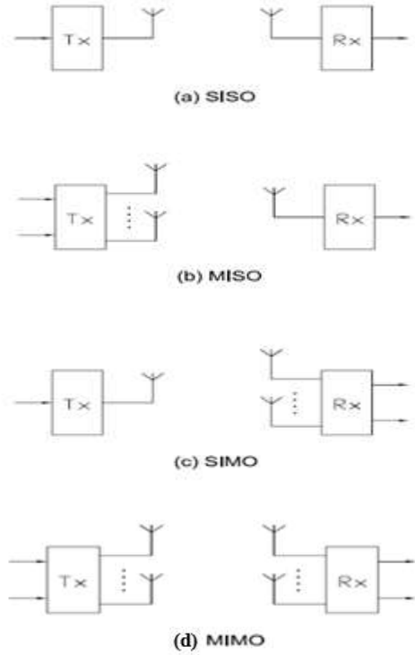
Figure 1: Antenna Configurations
