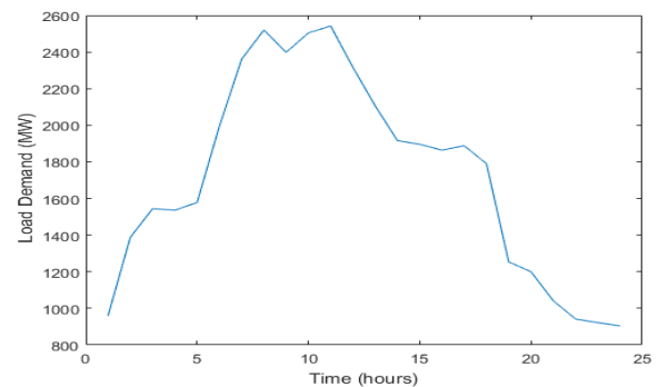
Fig. 4: Load demand profile
