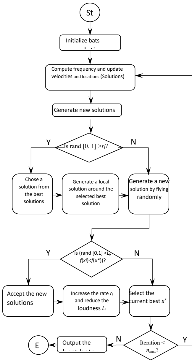
Fig. 1 The flowchart of ABIA technique (Elsisi et al., 2016)
