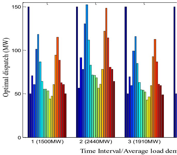
Fig. 5 Optimal dispatch of thermal generators
