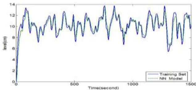
Figure 4.3 : NN Model and Training Data Evaluation
