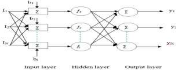
Figure 2. 1: NARX Model Layers Description
