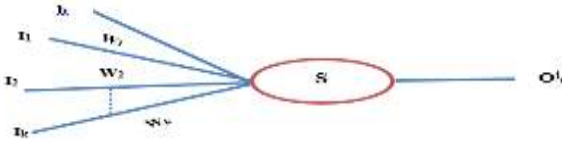
Figure 2.2. Neuron Model
