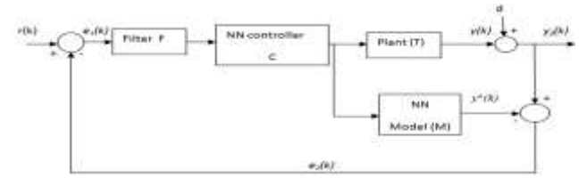
Figure 3.1: NNIMC Control Strategy
