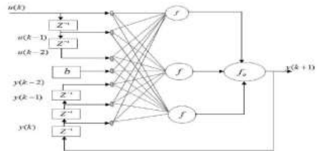
Figure2.3 :NARX Model Structure
