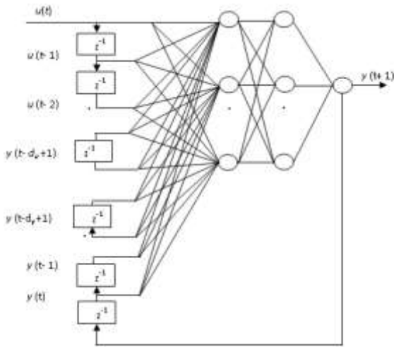
Fig. 3. NARX Architecture with Input d_u and Output d_y Tapped Delays
