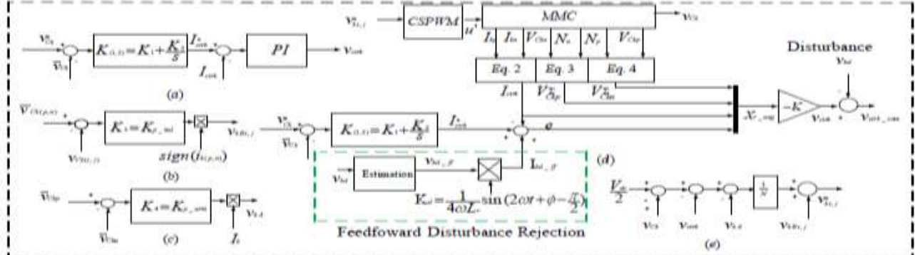
Fig. 2. Internal control of the CSPWM based MMC inverter (a) Conventional averaging capacitor voltage-circulating current control (b) Individual voltage balancing (c) Arm balancing control (d) Proposed averaging capacitor voltage-circulating current control (e) Overall voltage command generation.
