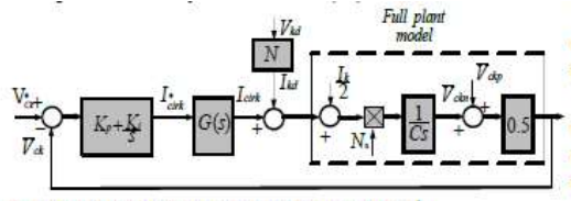
Fig. 3. Full model of average capacitor voltage control
