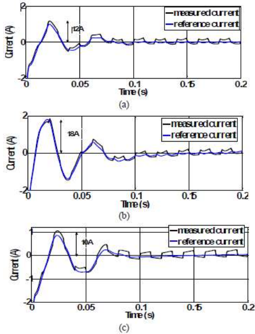
Fig. 6. Simulation waveform of the circulating current (a) based on the PI control method (b) based on the state-feedback method (c) based on the proposed state-feedback with the virtual impedance-loop method.
