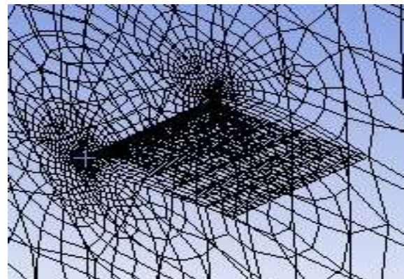
Plate IV: Mesh around the conventional blade
