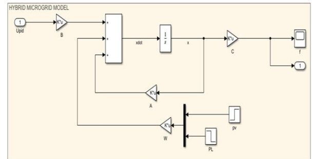
Figure 2: Hybrid Microgrid Model
