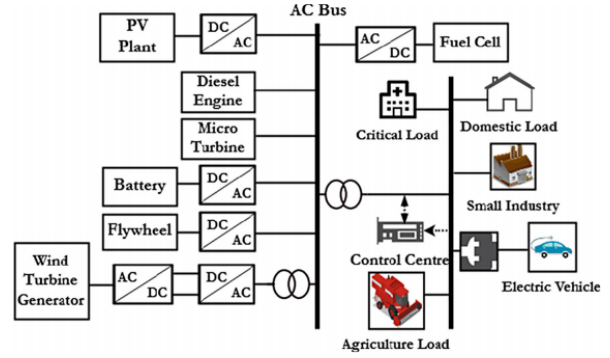
Figure 1: Microgrid Structure [25]
