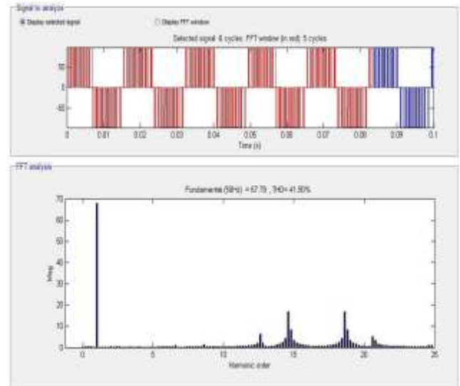
Fig 4.4 (b) Line Voltage Waveform and Harmonic Contents of 5-Level H-NPC Inverter at m_a = 0.2
