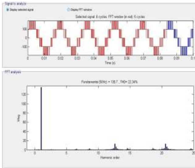
Fig 4.5(b) Line Voltages: Waveform and Harmonic Contents of 5-Level H-NPC Inverter at m_a = 0.4
