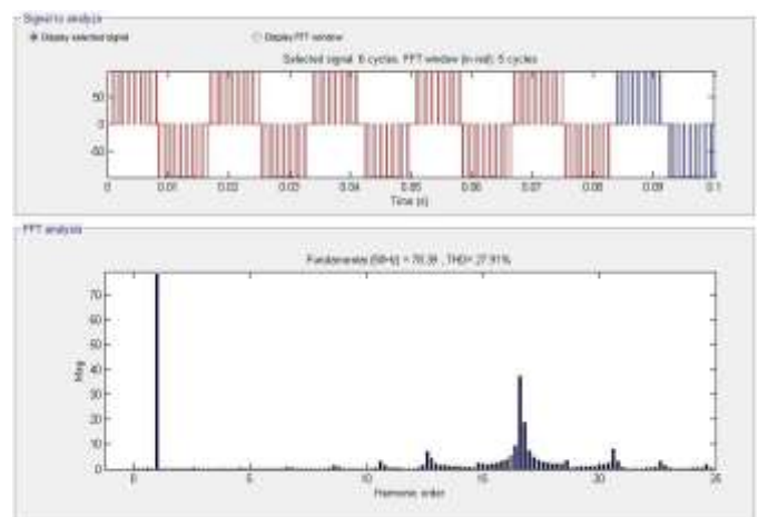
Fig 4.5(a): Phase Voltage Waveform and Harmonic Contents of 5-Level H-NPC Inverter at m_a = 0.4
