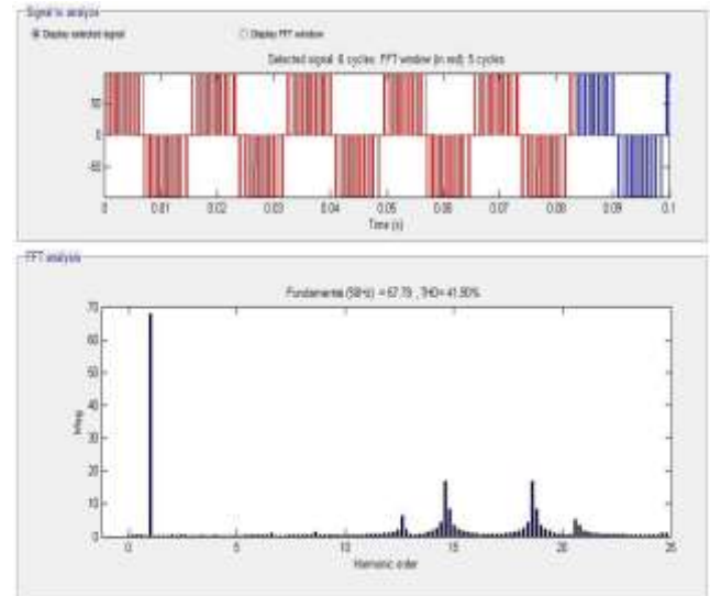
Fig 4.4 (b) Line Voltage Waveform and Harmonic Contents of 5-Level H-NPC Inverter at m_a = 0.2
