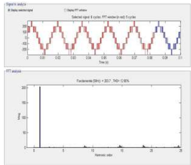
Fig 4.6(b) Line voltage: Waveform and harmonic contents of 5-level H-NPC inverter for m_a = 0.6
