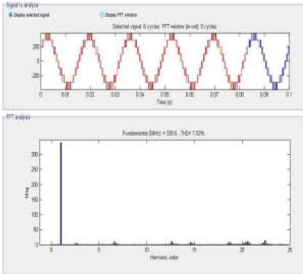
Fig 4.7(b) Line Voltage: Waveform and Harmonic Contents of 5-Level H-NPC Inverter at m_a = 1.0
