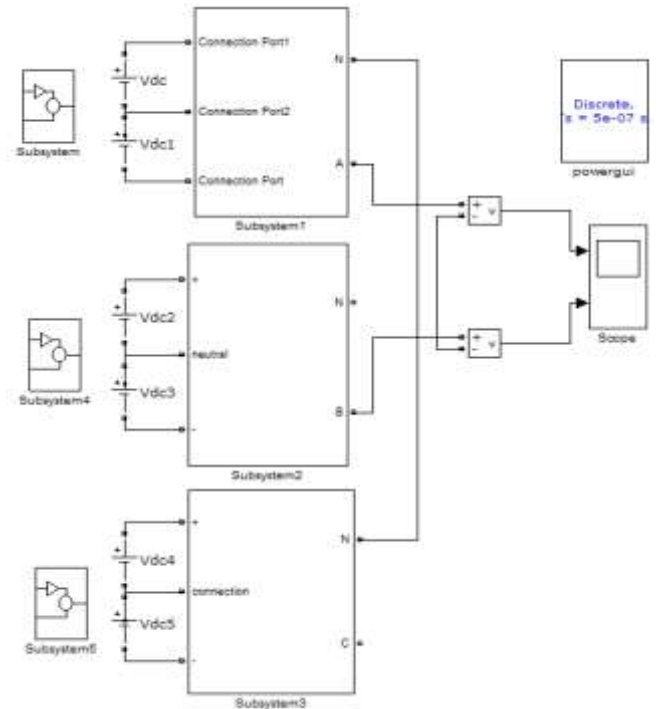
Fig 4.2 Three Phase 5-Level H-NPC Inverter Simulation Model
