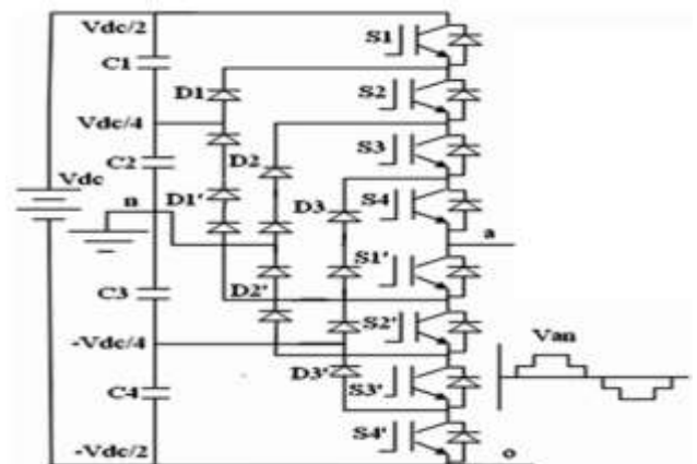
Fig 1.0 Single Phase Five Level Diode Clamp Inverter.
