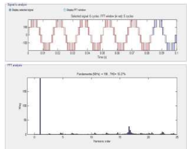
Fig 4.7(a): Phase Voltage Waveform and Harmonic Contents of 5-Level H-NPC Inverter for m_a = 1.0
