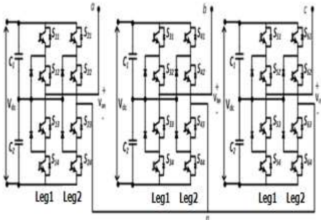
Fig.2.0 Three Phase Five Levels H-NPC Inverter Circuit Diagram [13]
