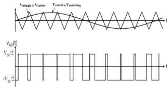
Fig 3.0(b). SPWM Output Waveform for Single Phase Two Level Voltage Source Inverter [6]
