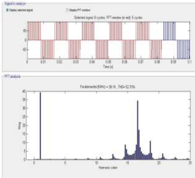
Fig 4.4(a): Phase Voltage Waveform and Harmonic Contents of 5-Level H-NPC Inverter at m_a = 0.2
