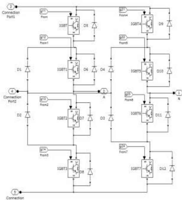
Fig. 4.1 Internal Circuitry of Phase 'a' Subsystem1 of 5 Level H-NPC Inverter
