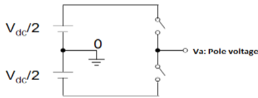
Fig. 3.0(a) Circuit Diagram for Single Phase Two Level Voltage Source Inverter [6]
