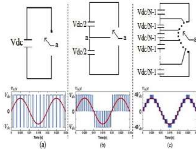
Fig. 1.1 Single phase Inverters and their output voltage waveform (a) “two level”, (b) “Three level”. (c) “N-levels” [6], [5]
