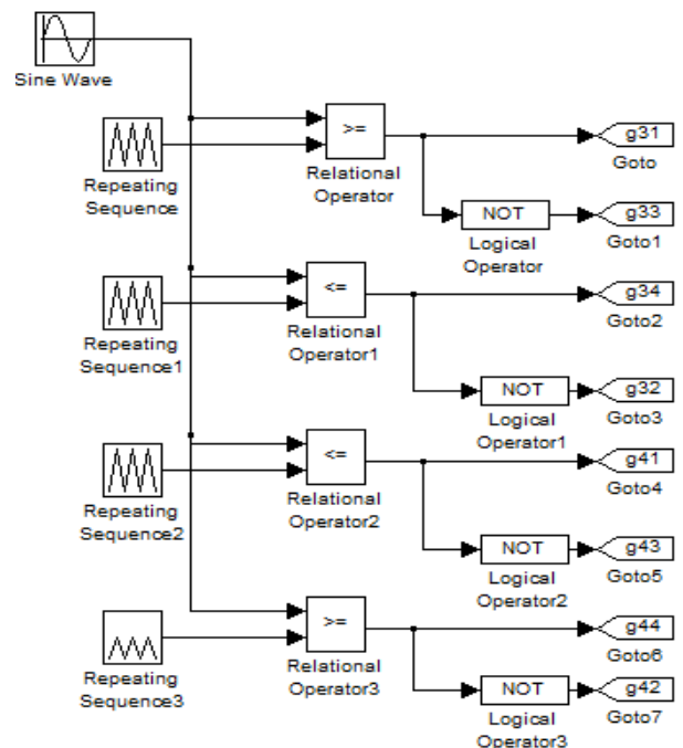
Fig 4.3 SPWM Simulation Block of 5-Level H-NPC Inverter in Phase 'a',
