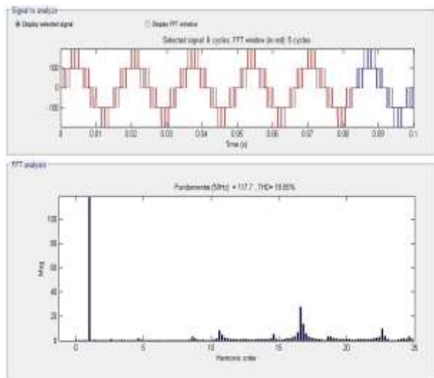
Fig 4.6 (a)Phase Voltage: Waveform and Harmonic Contents of 5-Level H-NPC Inverter for m_a = 0.6
