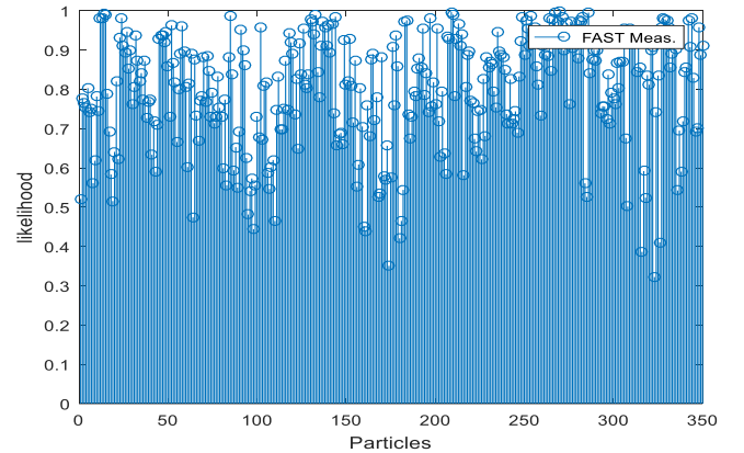
Figure 6 Likelihood Stem Plot of FAST Measurement
